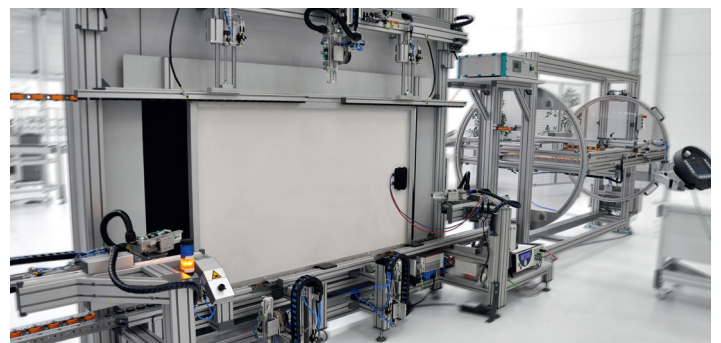
Backend-assembly line for photovoltaic-modules
